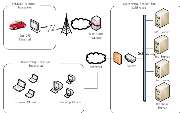
Fig. 2 Physical Structure of Shuttle Bus Monitoring Scheduling Subsystem
