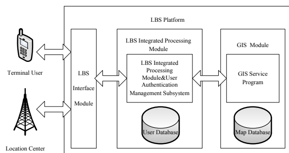
Fig. 1 The Overall Structure of LBS in OCT East
